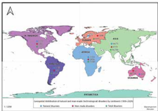
Prilog 1. Geoprostorna raspodela prirodnih i antropogenih (tehnoloških) katastrofa po kontinentima (1900–2024) (prema Cvetković et al., 2024). Figure 1. Geospatial distribution of natural and man-made (technological) disasters by continent (1900–2024) (according to Cvetković et al., 2024).
